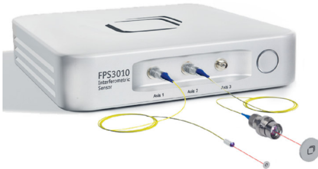
Figure 2: attocube's 3-axes real time interferometer, the FPS3010, features 25 \mu\text{m} resolution and a measurement bandwidth of 10 MHz. The fiber based measurement heads are available in sizes from 4 to 14 mm diameter dependent on the application. These heads are also compatible with ultrahigh vacuum as well as cryogenic conditions.
